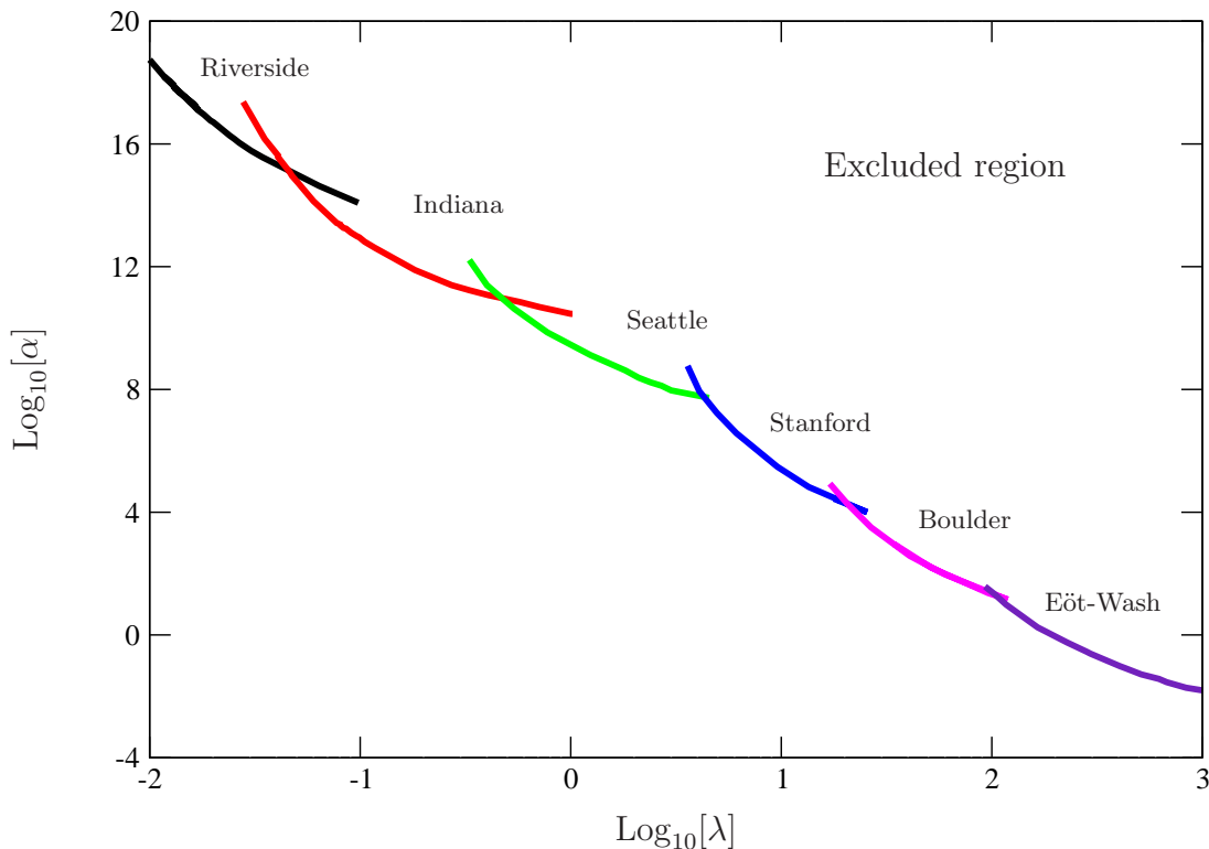
FIG. 3: Experimental constraints and predictions for a hypothetical Yukawa force in the \alpha - \lambda plane, with \lambda expressed in micrometres. The plot may be considered a prolongation of the \alpha - \lambda plot of Fig. 1 on the upper left corner. The excluded region is delimited by curves compatible with no Yukawian-signal in the measured data within two standard deviations. From left to right, limits coming from three experiments on Casimir forces performed in the 100 nm-1 \mu\text{m} range at room temperature [84, 94, 117], two experiments with microresonators operating in the 100 \mu\text{m} distance range [18, 19], and one experiment using a torsion pendulum with rotating attractor [15], are shown.
